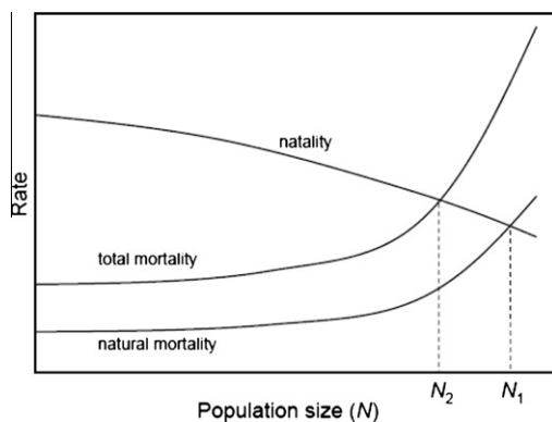
Fig. 8. Population growth as a function of density-dependent mortality and natality. Natural mortality occurs in the absence of anthropogenic mortality, whereas the difference between natural mortality and total mortality represents additive effects of anthropogenic mortality. Anthropogenic mortality is functionally density-dependent at high population density, and reduces equilibrium population density from N_1 to N_2 . Adapted from Boyce et al. (1999).
